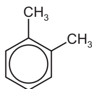
1,2-dimethylbenzene
