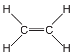
ethene
